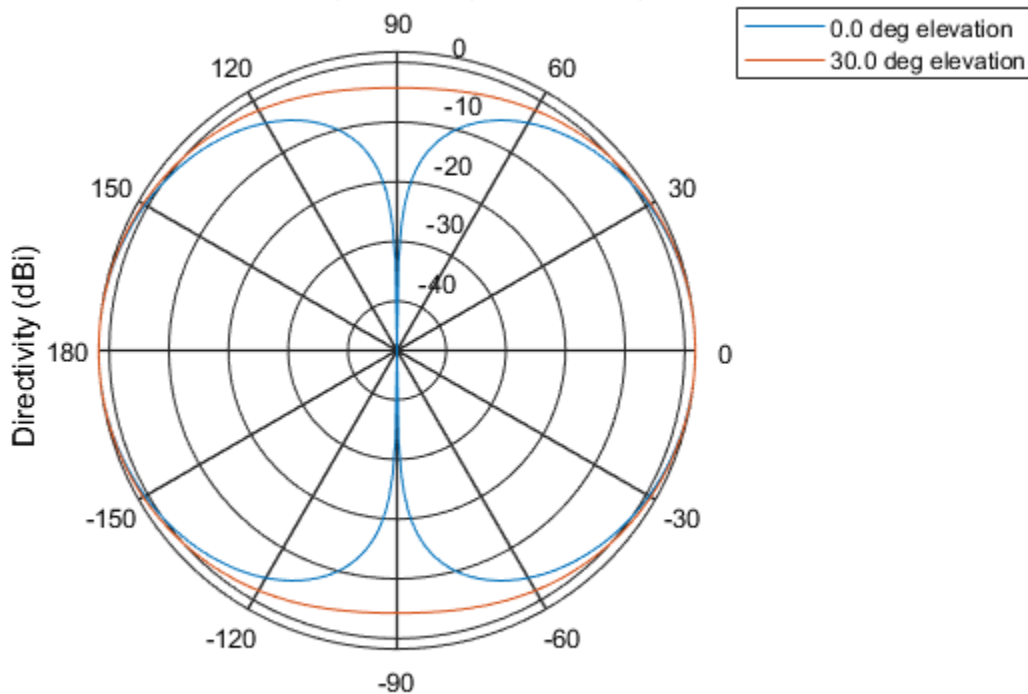
Azimuth Cut (frequency = 500 MHz)
