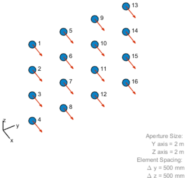
Array Geometry
